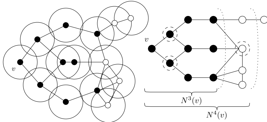
Fig. 1. Example of a UDG with and without geometric representation
