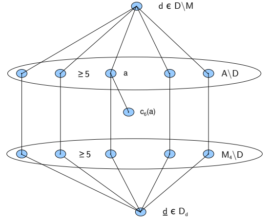
Figure 7: Substructure of H analyzed in Proposition 4.11. Observe that nodes of M_6 \setminus D can also be in M_4 \setminus D .
